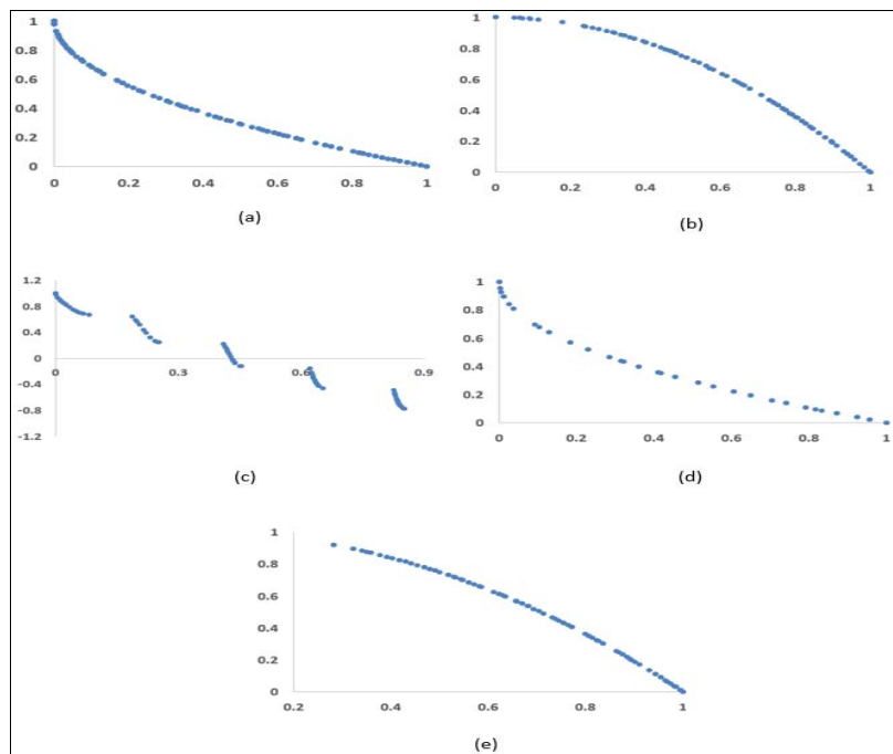
Fig. 11. Obtained POE by the proposed algorithm. a: ZDT1, b: ZDT2, c:ZDT3, d:ZDT4, e:ZDT6
