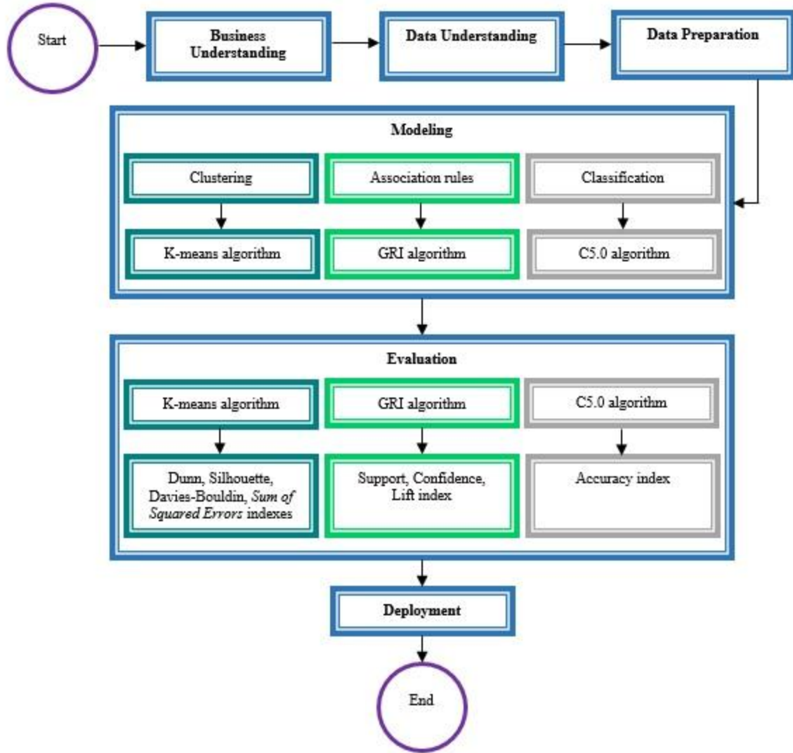
Fig 1. Procedure of research
