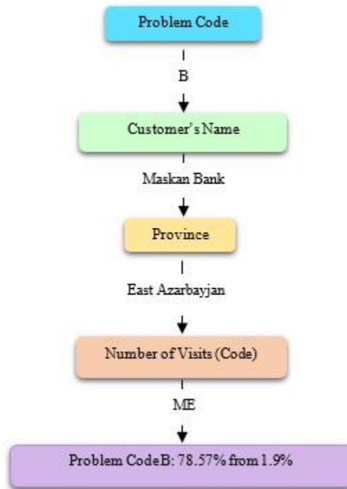
Fig 2. The procedure of extraction rule number one
