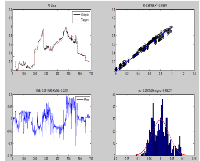
Fig. 5. Neural network output diagrams for Razak Pharmaceutical Company as the worst ranking.
