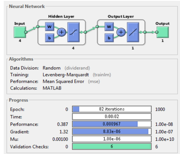
Fig. 2. Neural network learning process
