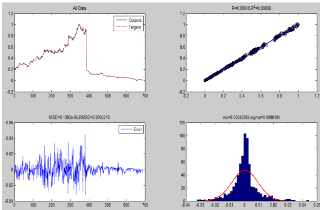
Fig. 3. Neural network output diagrams for Dr. Abidi Pharmaceutical Company as the best ranking
